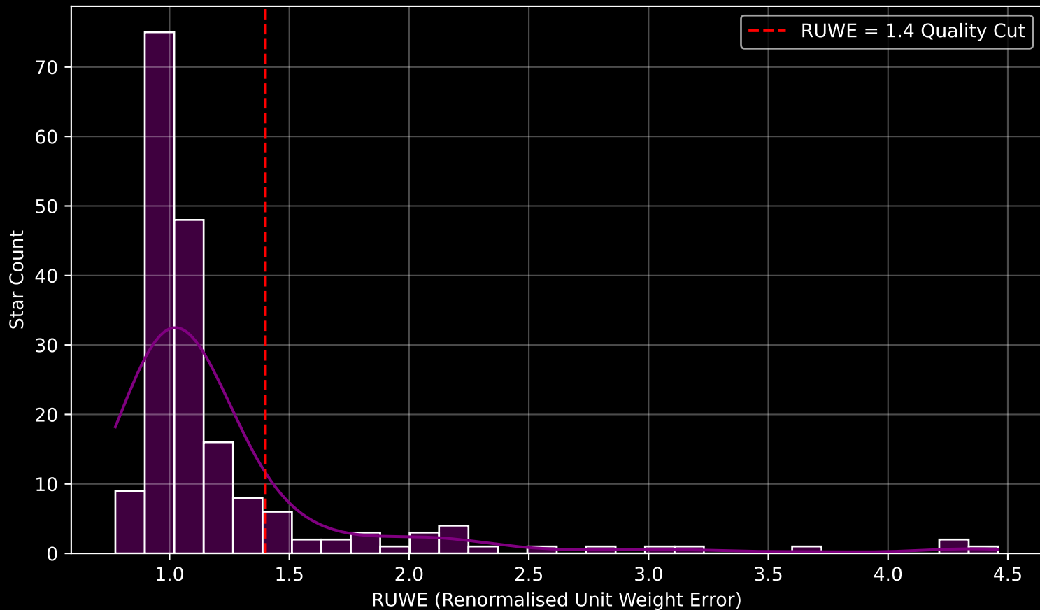
GAPOGEE DR17 Field [196+35_MGA] RUWE Distribution (n= 186)
