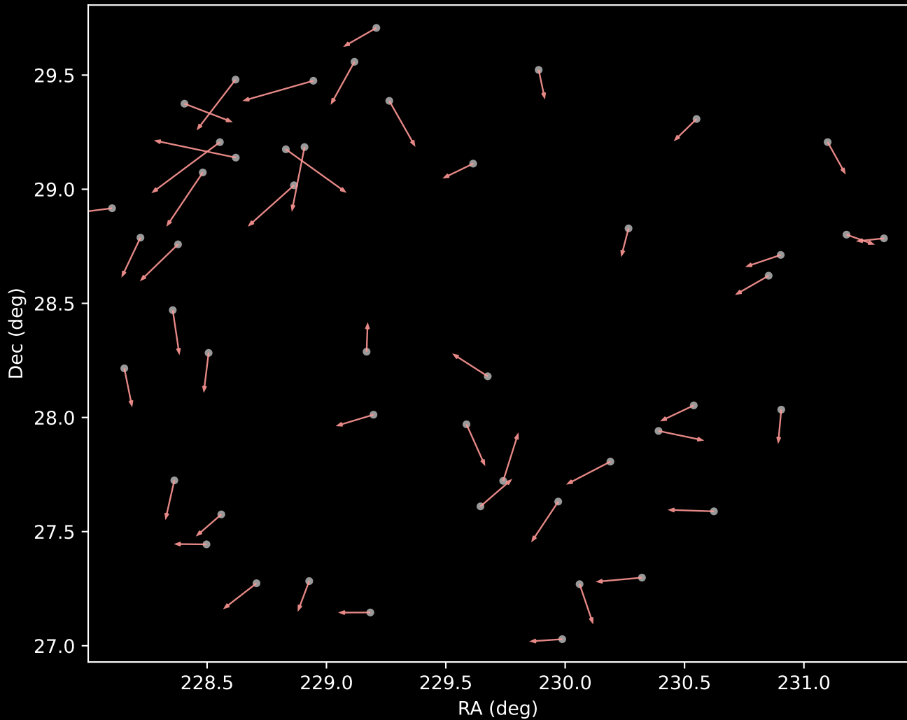
APOGEE DR17 Cluster 7 Proper Motion Vectors (n=48)
