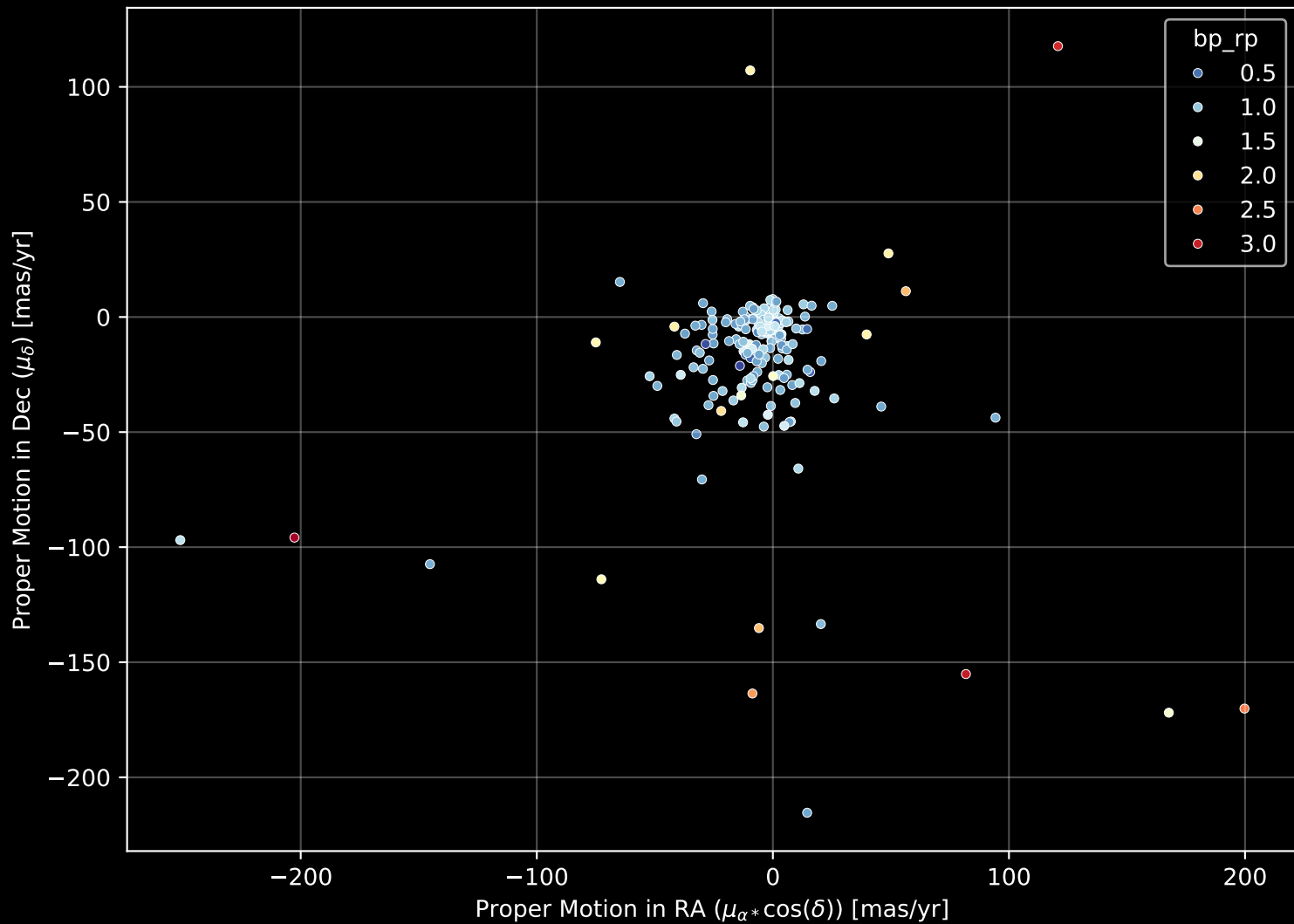
APOGEE DR17 Field: [196+35_MGA] Proper Motion Diagram (n= 198)
