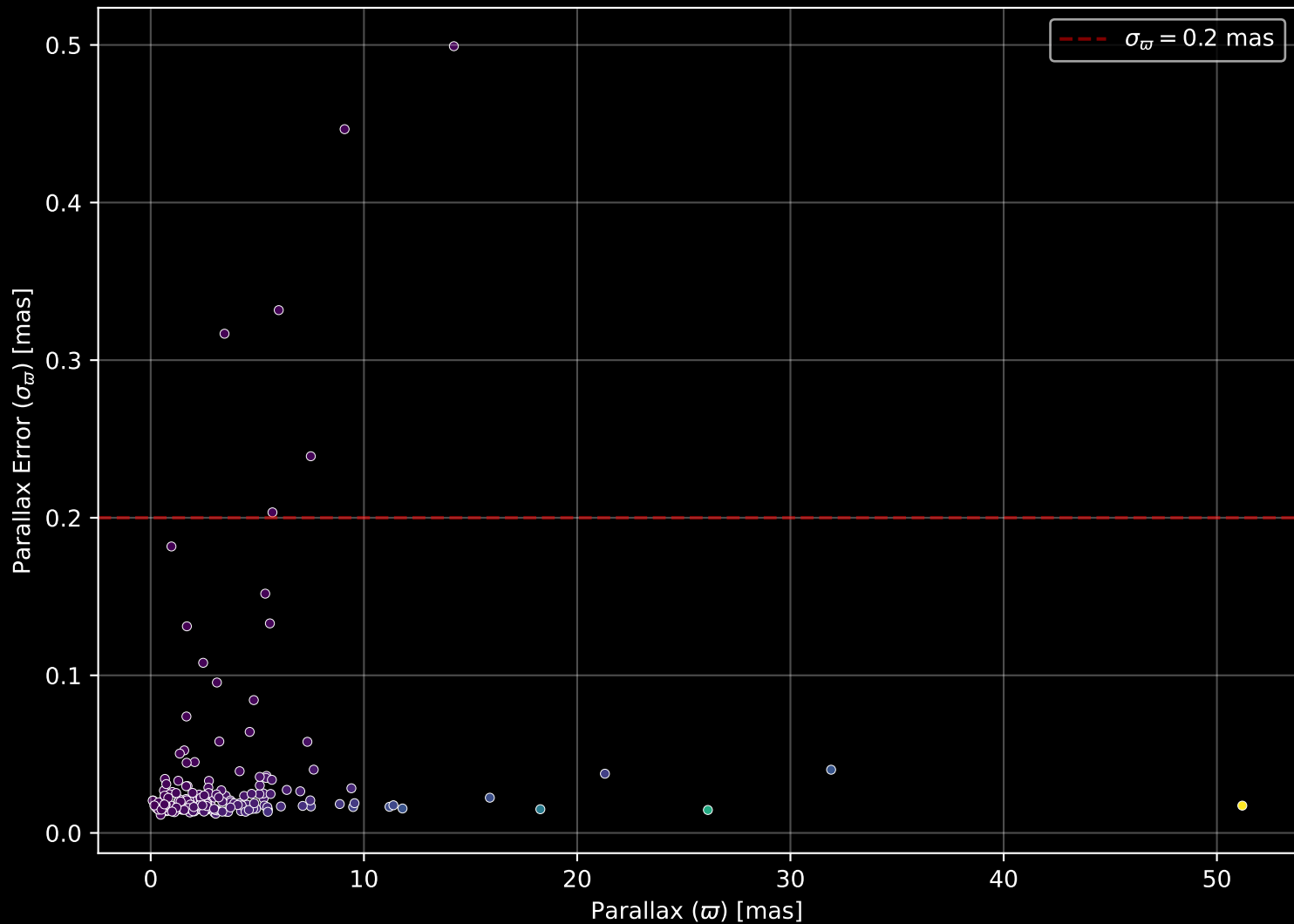
APOGEE DR17 Field: [196+35_MGA] Parallax Quality (n= 198)
