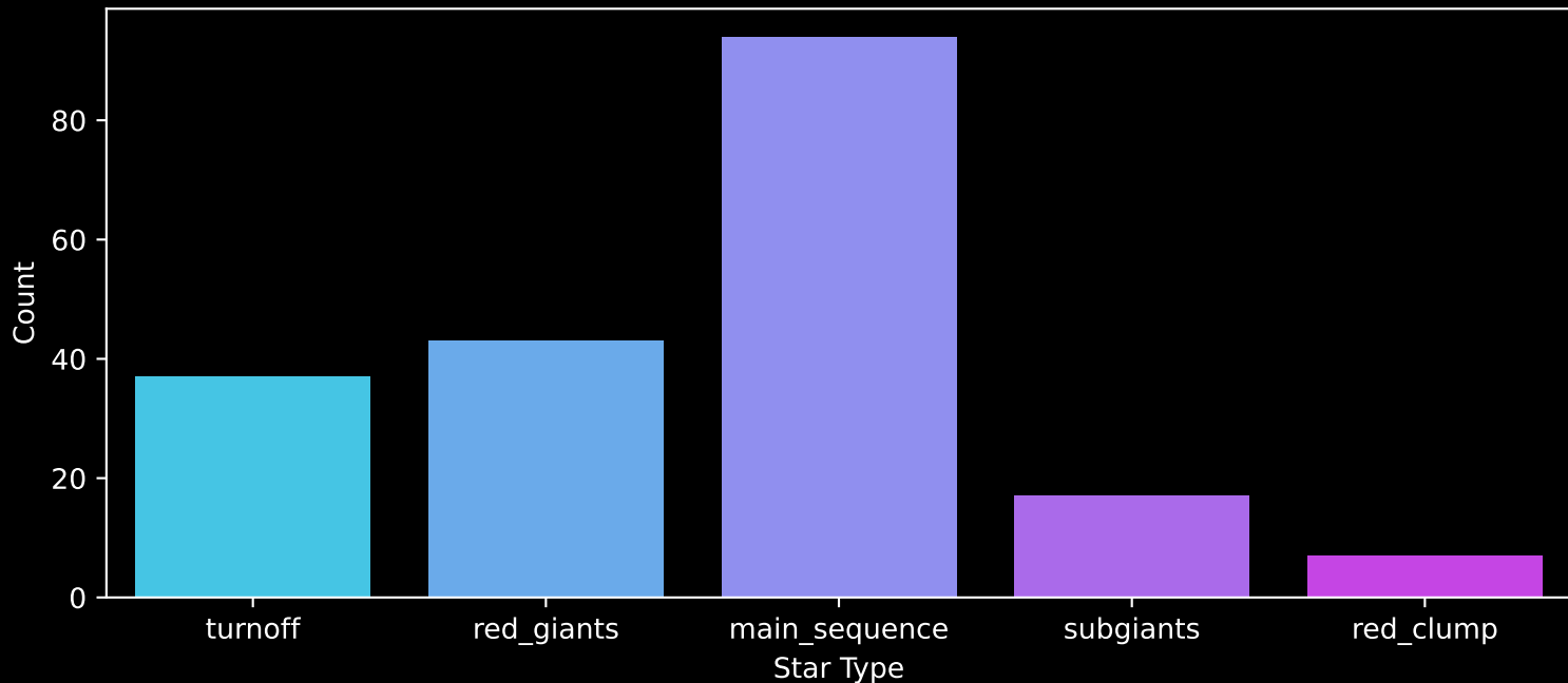
APOGEE DR17 Field: [196+35_MGA] Count plot of Star Type
