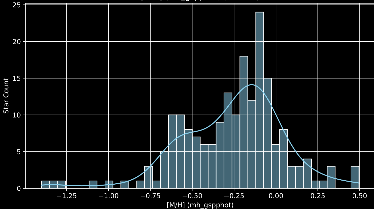
APOGEE DR17 Field: [196+35_MGA [M/H] (mh_gspphot) (n= 196)
