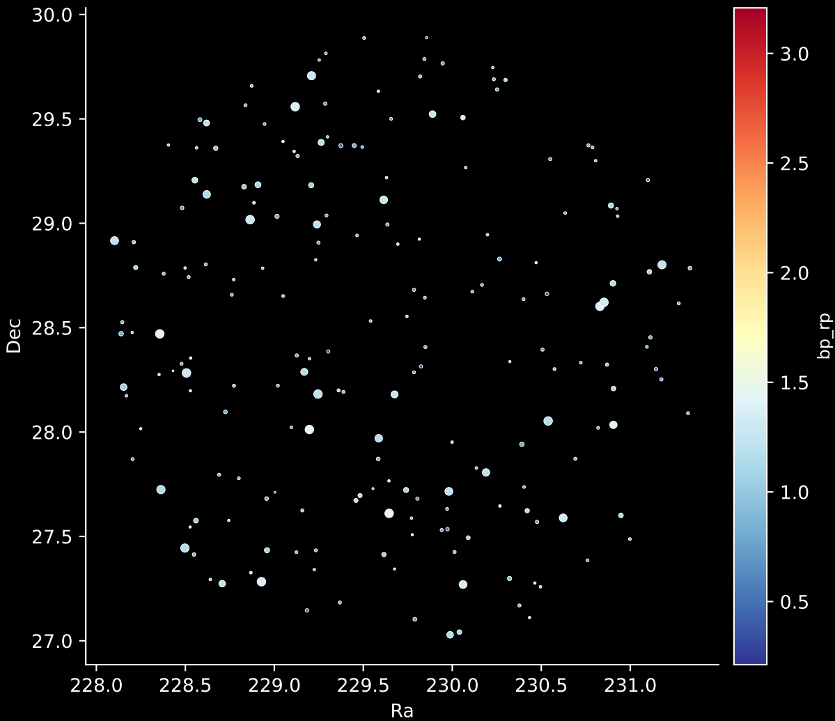
APOGEE DR17 Field: [196+35_MGA] Stars: 198
